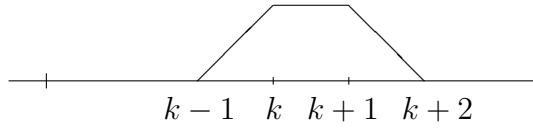
Figure 3: Symmetric trapezoidal hedge (positive side only)
