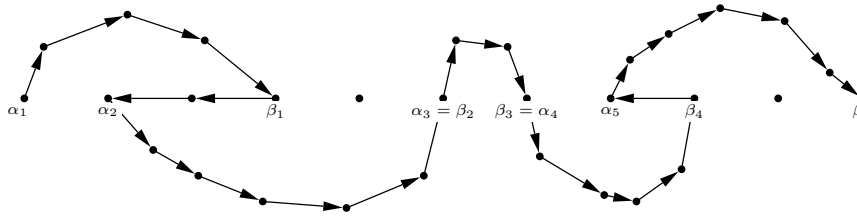
Figure 15: Directed path in \widetilde{G}' .
