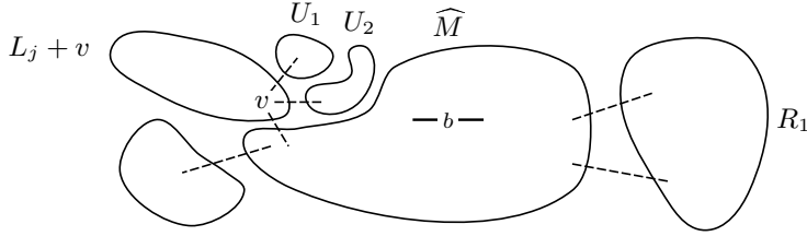
Figure 9: Cut conjunction K in (q2-c)
