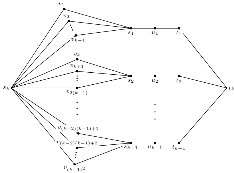
Figure 1: Minimal B -cuts contain exactly one edge of each pair s_i u_i and u_i t_i , for i = 1, \dots, k - 1 , thus we have |\mathcal{F}| = 2^{k-1} . On the other hand, the number of minimal s_k - t_k cuts is more than 2^{(k-1)^2} , so it is not polynomially bounded by |V| = k^2 + k and |\mathcal{F}| .
