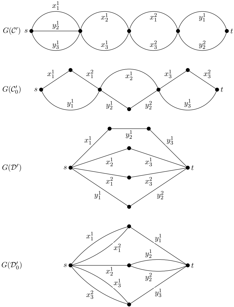
Figure 4: Four labeled graphs corresponding to the CNF \mathcal{G} .
