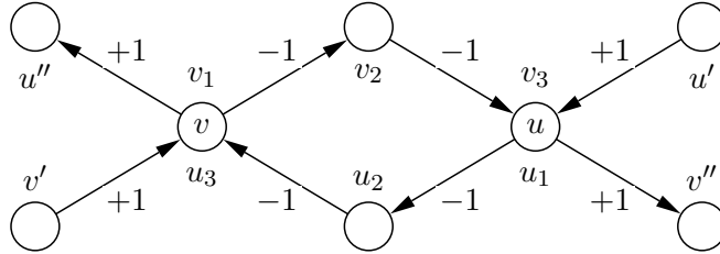
Figure 5: Two pairs of vertices are merged.
