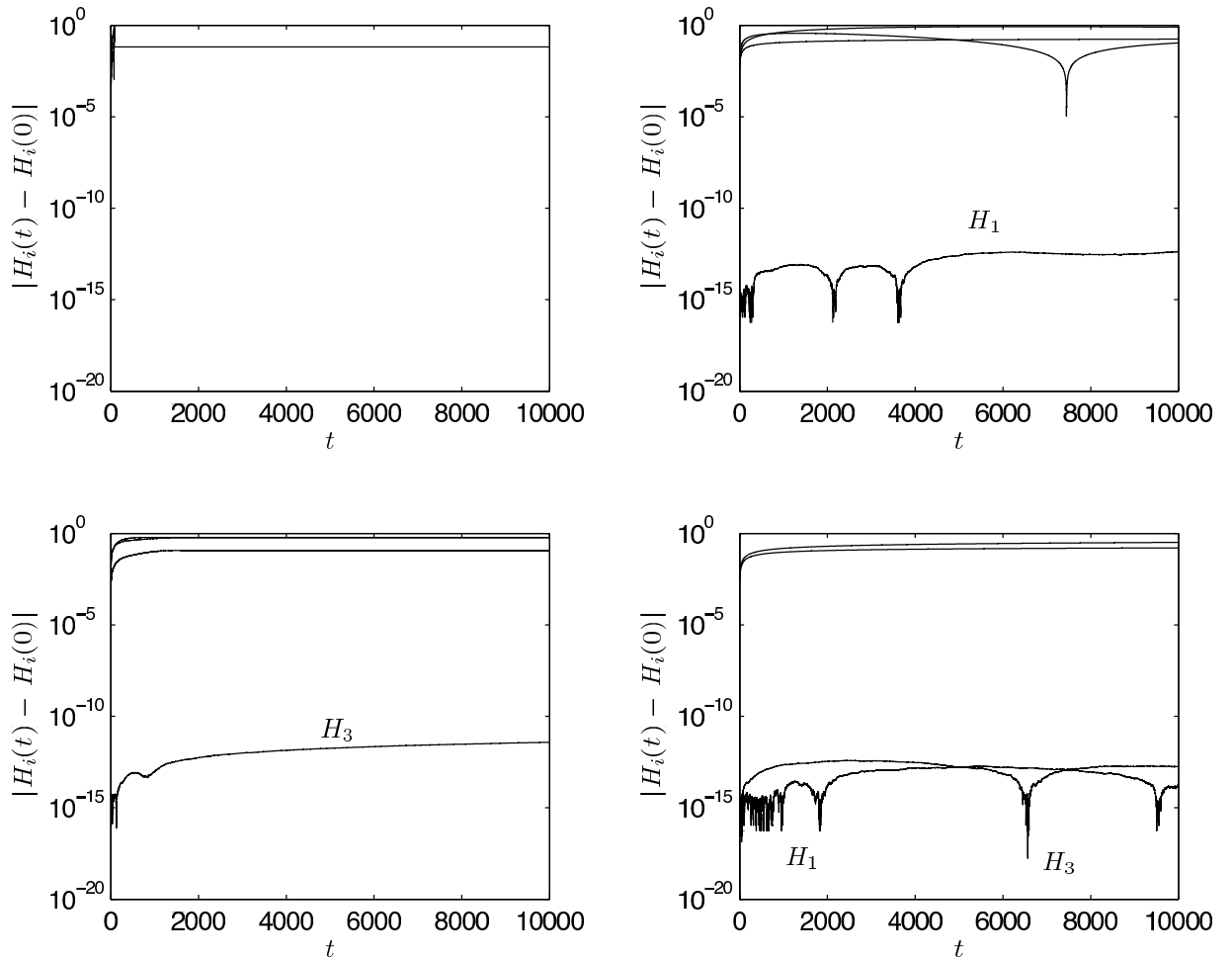
Fig. 2 The error in the first integrals for the solutions of the four schemes of Table 1. There is one line for each of the four invariants. 50000 steps are shown.
