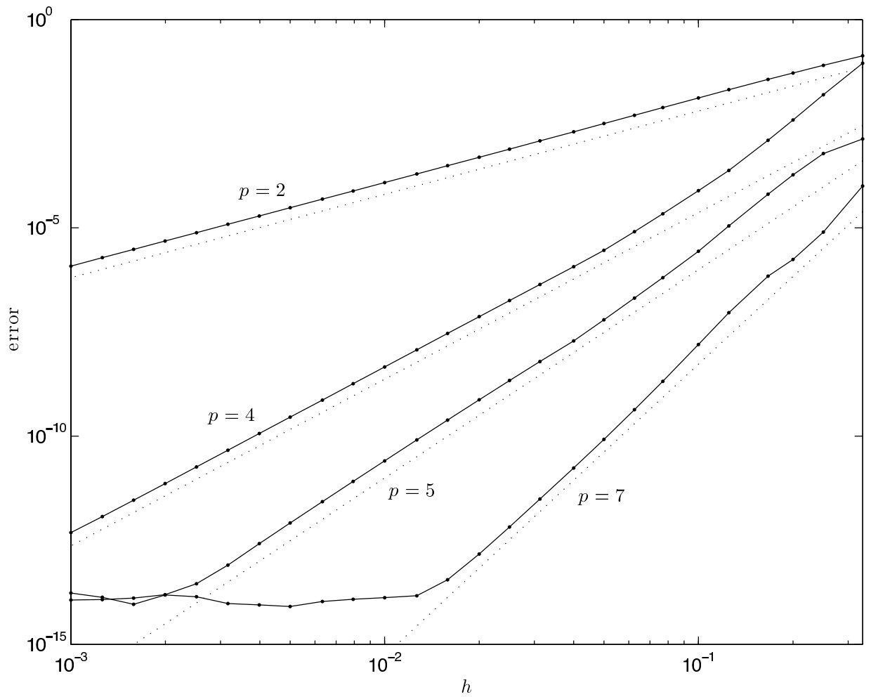
Fig. 3 The global error of the four schemes RK2Proj123, RK4Proj123, RK5Proj123, and RK7Proj123. The dotted lines are reference lines of exact order.
