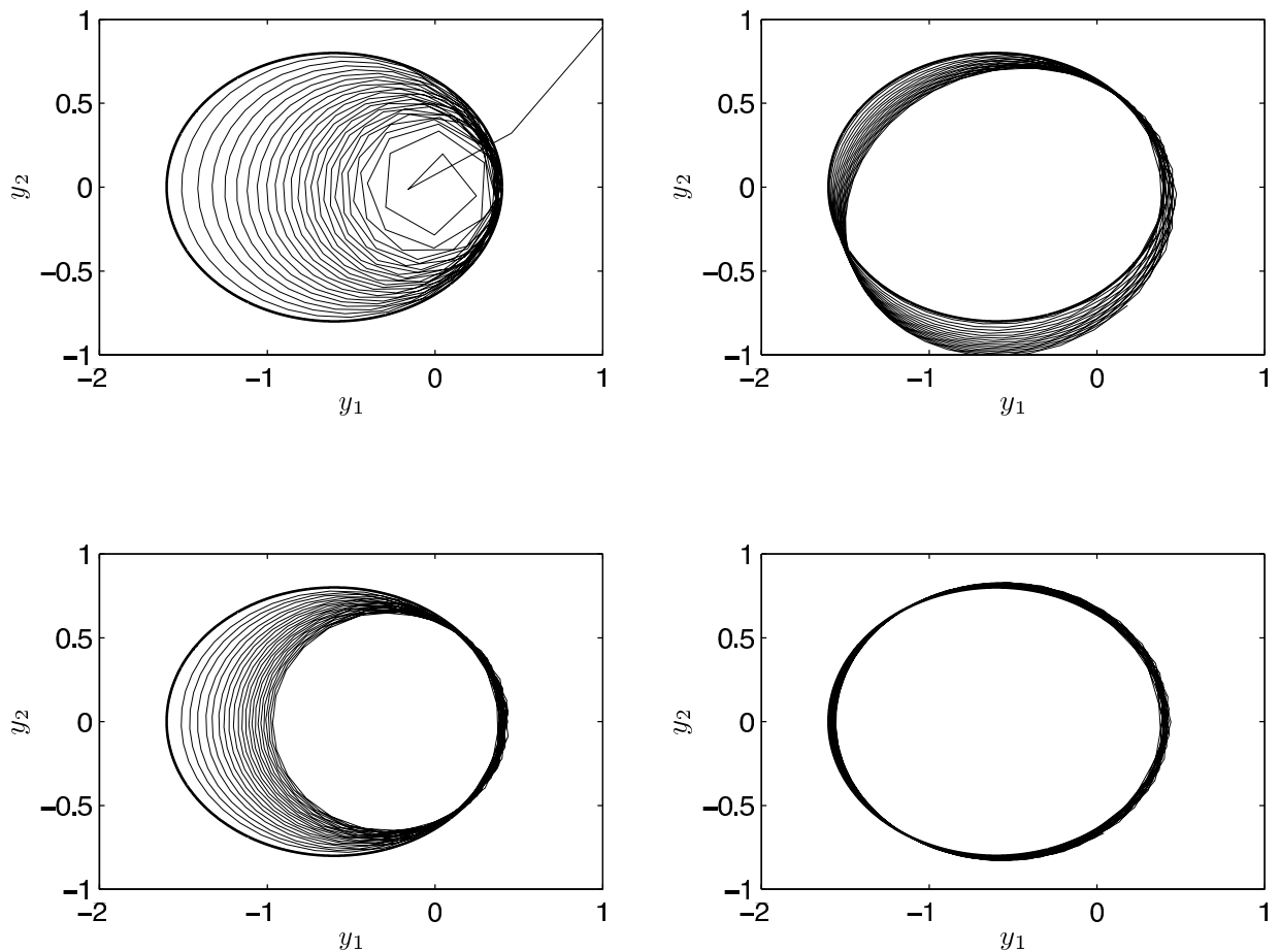
Fig. 1 The numerical solution (thin line) of the Kepler problem (3.1) using the schemes of Table 1 with h = 0.2 . The first 500 steps are shown. The exact solution (thick line) is an ellipse with eccentricity e = 0.6 .
