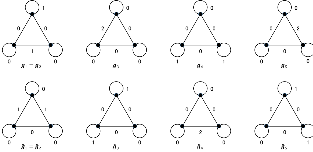
Figure 7: Graphs \mathbf{g}_1 = \mathbf{g}_2, \mathbf{g}_3, \mathbf{g}_4, \mathbf{g}_5 and \hat{\mathbf{g}}_1 = \hat{\mathbf{g}}_2, \hat{\mathbf{g}}_3, \hat{\mathbf{g}}_4, \hat{\mathbf{g}}_5
